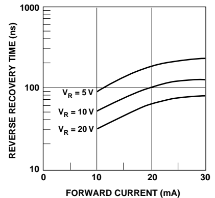
Figure 9. Typical Reverse Recovery Time vs. Forward Current for Various Reverse Driving Voltages, 5082-3140.
