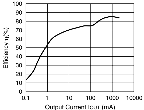
R1225N182B (VIN=5.0V) CDRH127-10uH
