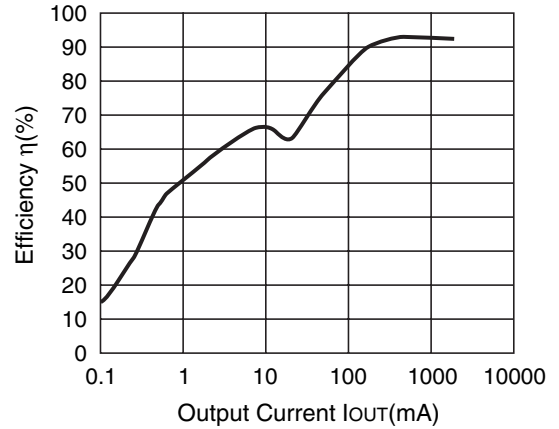
R1225N332B (V IN =4.8V) CDRH127-10uH
