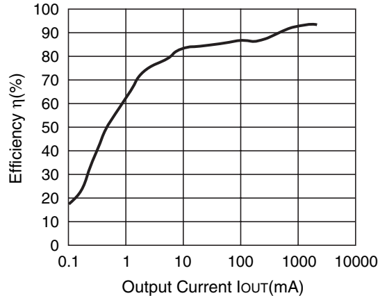
R1225N502A (V IN =10V) CDRH127-10uH
