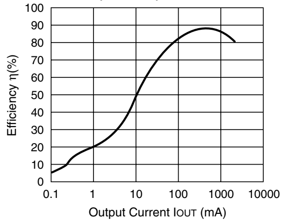
R1225N182D (V IN =3.3V) CDRH127-10uH
