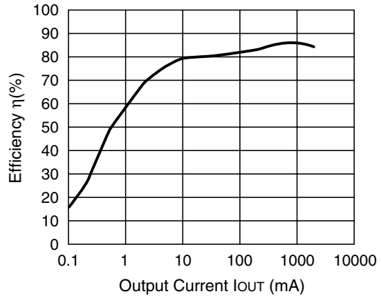
R1225N182B (VIN=5.0V) CDRH127-10uH
