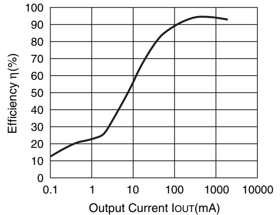
R1225N332C (V IN =4.8V) CDRH127-10uH
