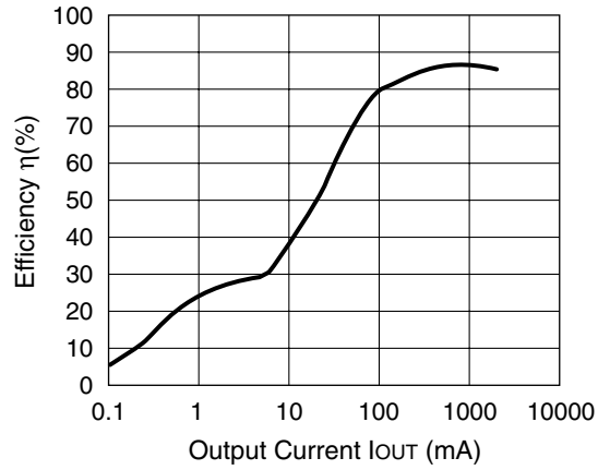
R1225N182C (V IN =5.0V) CDRH127-10uH
