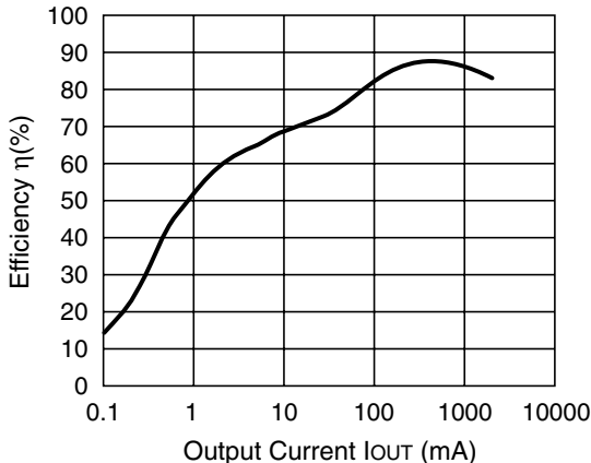
R1225N182B (VIN=3.3V) CDRH127-10uH
