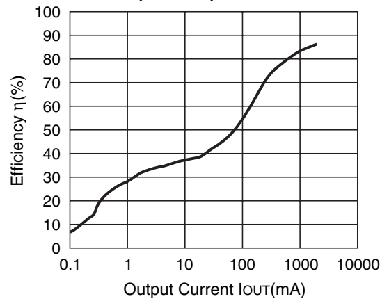
R1225N332C (V IN =15V) CDRH127-10uH
