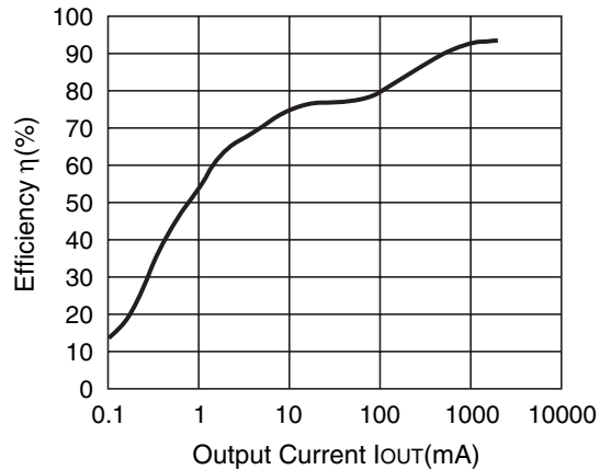
R1225N502B (V IN =10V) CDRH127-10uH
