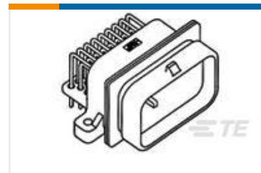
TE Part #6437288-2 SUPER SEAL 34POS CAP ASSY
