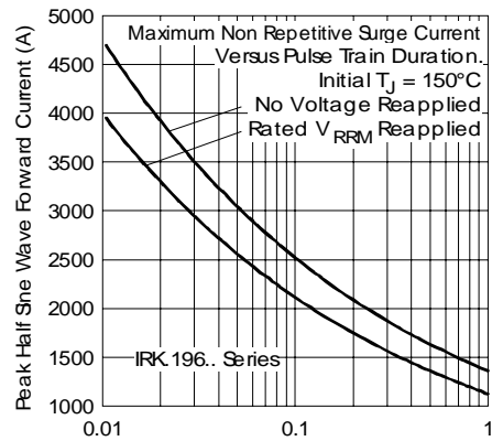
Fig. 15 - Maximum Non-Repetitive Surge Current
