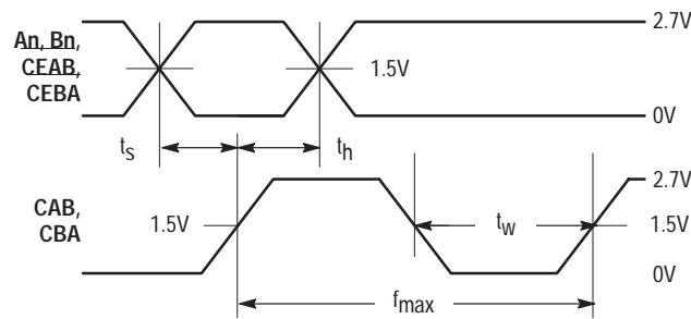
WAVEFORM 3 – Cxx MINIMUM PULSE WIDTH, An/Bn/CExx to Cxx SETUP AND HOLD TIMES t_R = t_F = 2.5ns, 10\% \text{ to } 90\%; f = 1MHz; t_W = 500ns \text{ except when noted}
