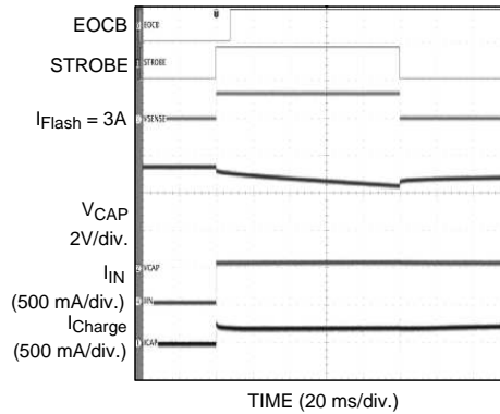
Figure 31. Level-Sensitive Strobe
