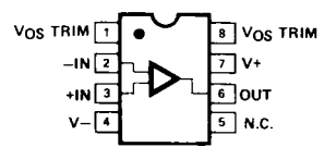
8-PIN HERMETIC DIP (Z-Suffix)
