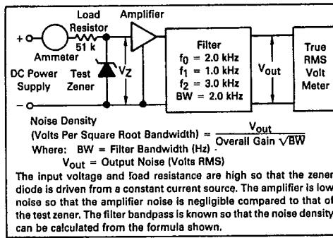
FIGURE 10 — NOISE DENSITY MEASUREMENT METHOD
