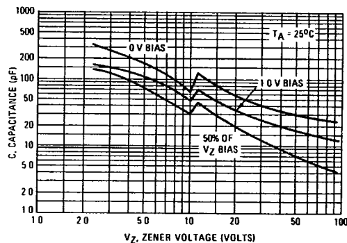
FIGURE 5 — TYPICAL CAPACITANCE
