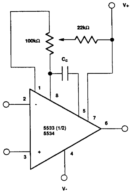
Frequency Compensation and Offset Voltage Adjustment Circuit
