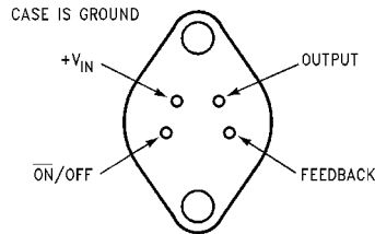
Bottom View LM1575K-XX or LM1575HVK-XX/883 See NS Package Number K04A
