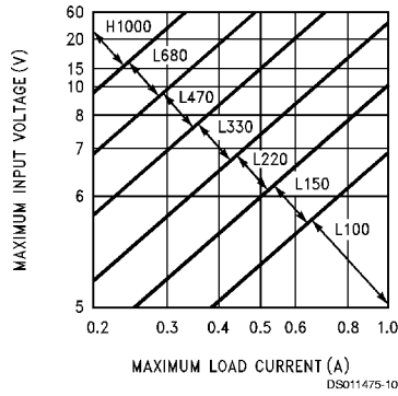
FIGURE 3. LM2575(HV)-3.3
