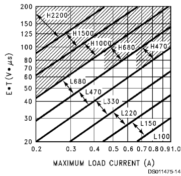
FIGURE 7. LM2575(HV)-ADJ
