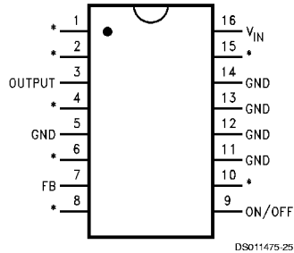
Top View LM2575N-XX or LM2575HVN-XX See NS Package Number N16A
