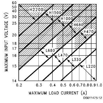
FIGURE 5. LM2575(HV)-12
