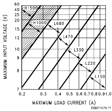
FIGURE 4. LM2575(HV)-5.0
