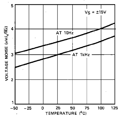
VOLTAGE NOISE DENSITY vs TEMPERATURE
