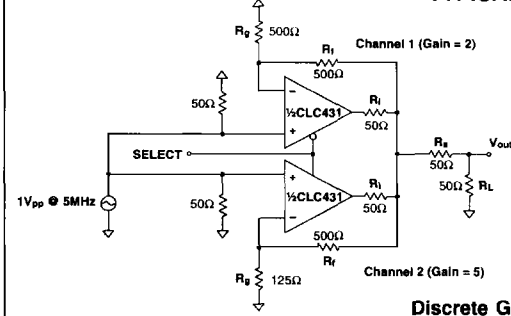
Discrete Gain Select Amplifier
