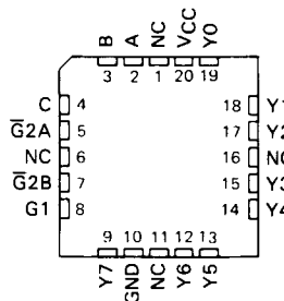
SN54ALS138, SN54AS138 . . . FK PACKAGE (TOP VIEW)
