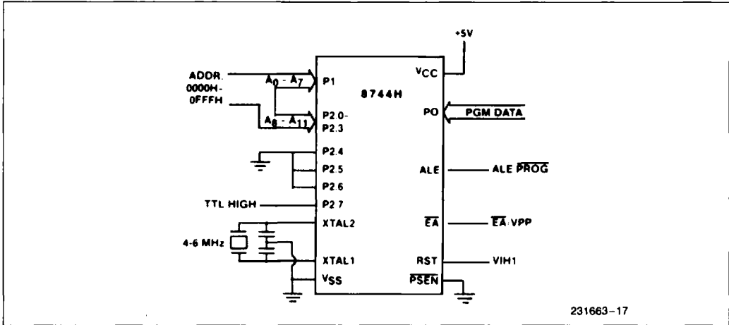
Figure 8. Programming Configuration
