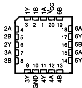
SN54ALS804A, SN54AS804B ... FK PACKAGE (TOP VIEW)
