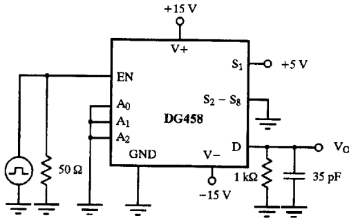
Figure 5. Enable Delay
