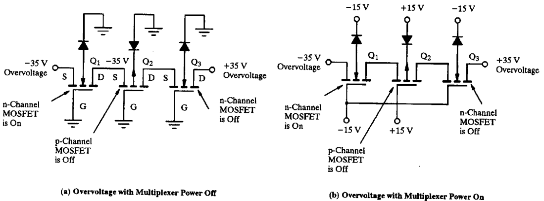
Figure 6. Overvoltage Protection
