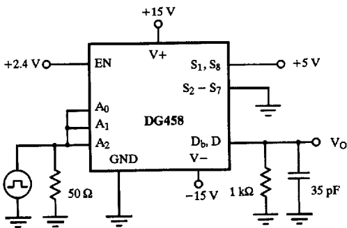
Figure 4. Break-Before-Make Time
