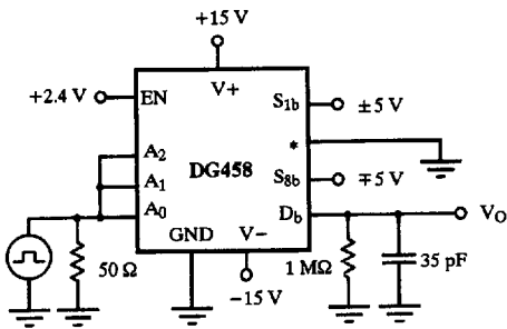
Figure 3. Transition Time
