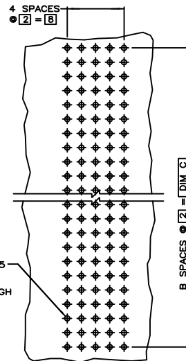
RECOMMENDED CIRCUIT PATTERN (COMPONENT SIDE)
