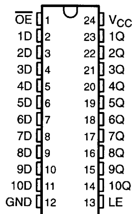
SN74ALS841, SN74AS841A . . . DW OR NT PACKAGE (TOP VIEW)
