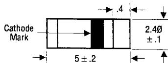
Glass case MiniMELF
