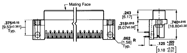
With Threaded Insert
