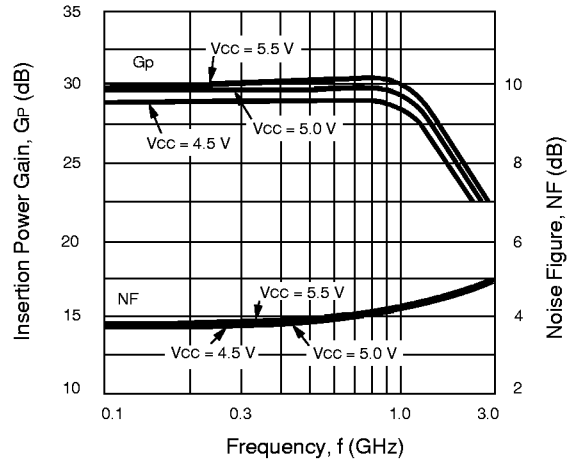
UPC2713T NOISE FIGURE AND INSERTION GAIN vs. FREQUENCY
