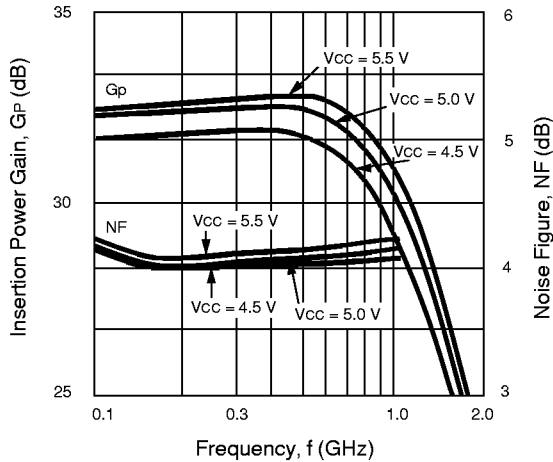
UPC2710T NOISE FIGURE AND INSERTION GAIN vs. FREQUENCY
