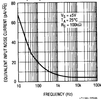
Equivalent Input Noise Current vs Frequency
