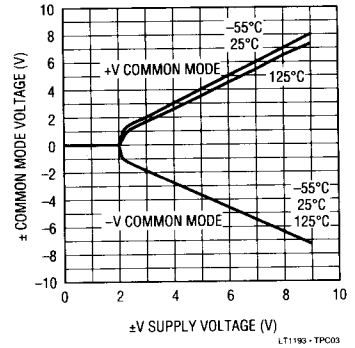
Common Mode Voltage vs Supply Voltage
