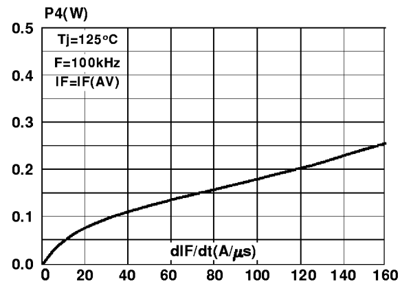
Fig 10 : Switching ON losses versus dIF/dt
