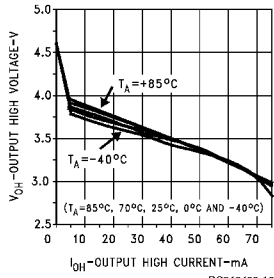
Driver V_{OH} vs I_{OH} vs Temperature
