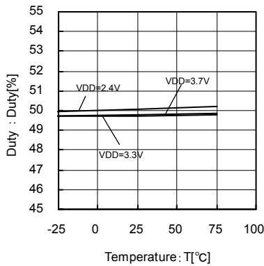
Fig.108 24.6MHz Temperature-Duty
