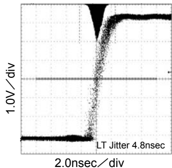
Fig.97 24.6MHz LT Jitter VDD=3.3V, at CL=15pF
