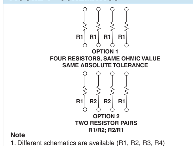
FIGURE 1 - SCHEMATICS 1)
