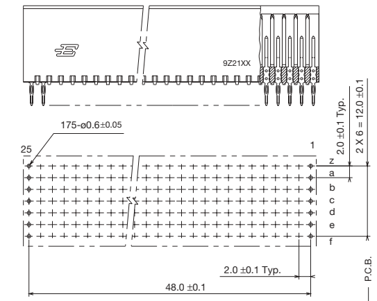
RECOMMENDED P.C. BOARD LAYOUT (COMPONENT SIDE)
