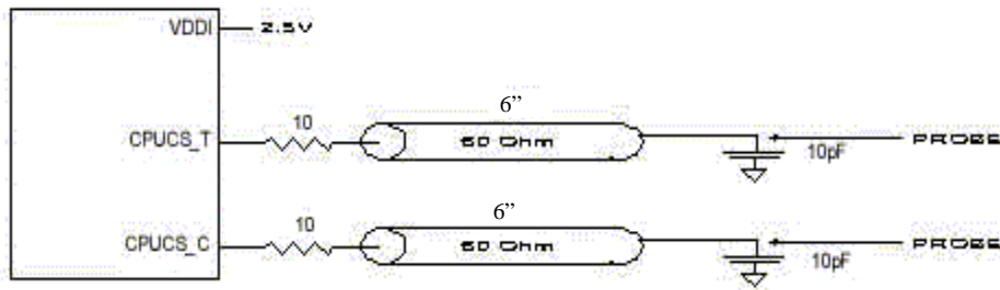
Figure 2. K7 Termination
