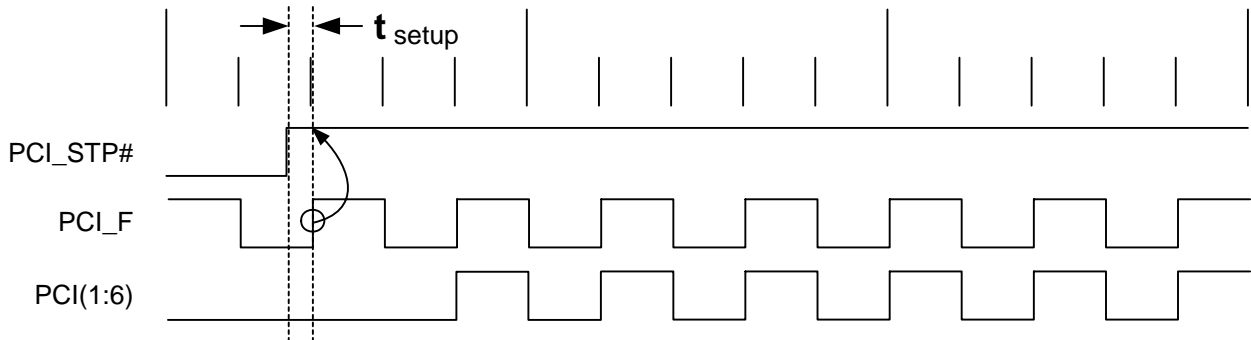
Figure 12. PCI_STP# Deassertion Waveform
