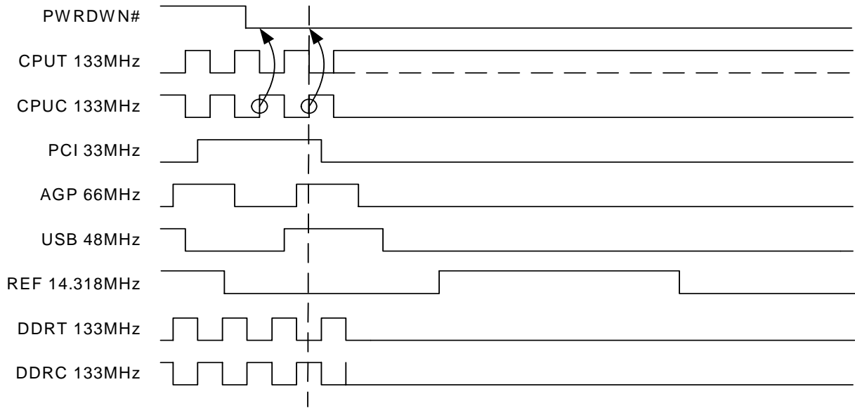
Figure 13. Power-down Assertion Timing Waveform (in P4 Mode)
