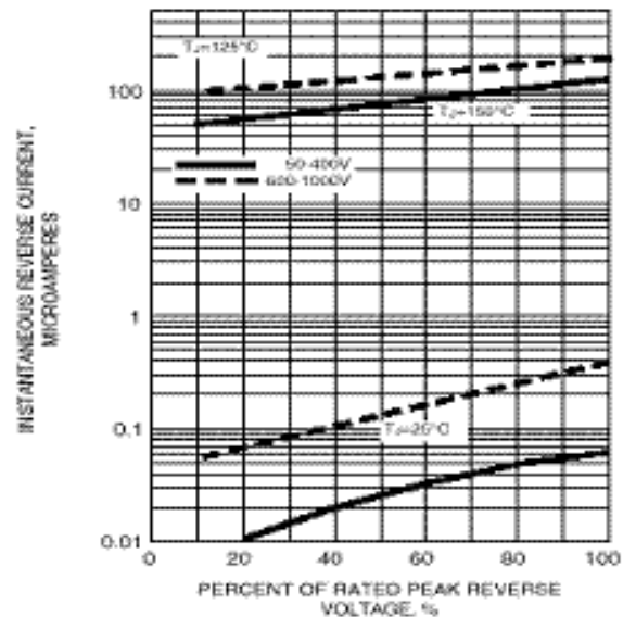
FIG. 6 - TYPICAL REVERSE LEAKAGE CHARACTERISTICS PER LEG
