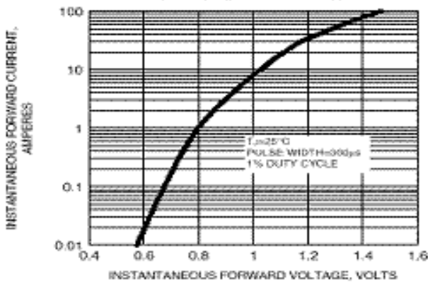
FIG. 5 - TYPICAL INSTANTANEOUS FORWARD CHARACTERISTICS PER LEG
