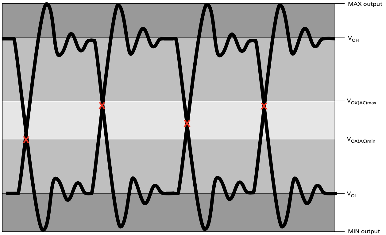
Figure 23: Differential Output Signal
