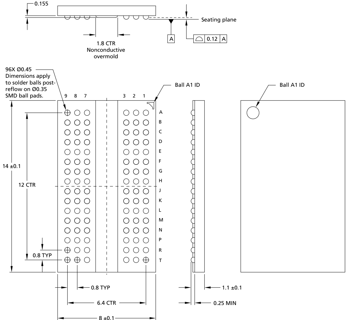
Figure 6: 96-Ball FBGA – x16 (JT)
