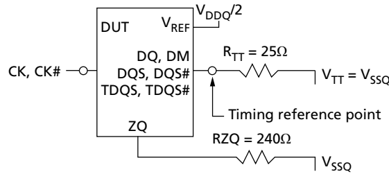
Figure 17: ODT Timing Reference Load
