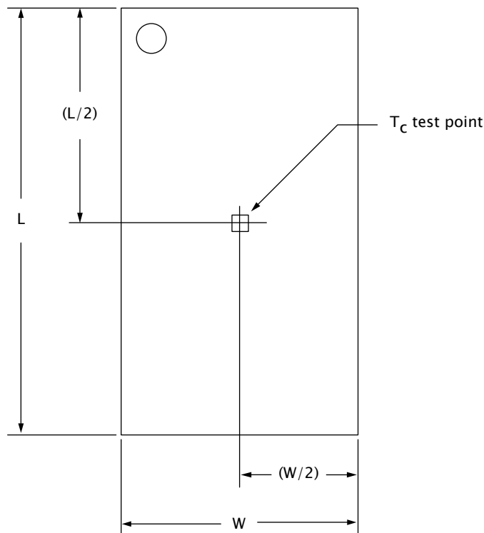
Figure 7: Thermal Measurement Point
