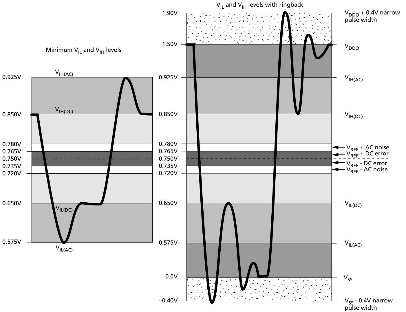
Figure 8: Input Signal
