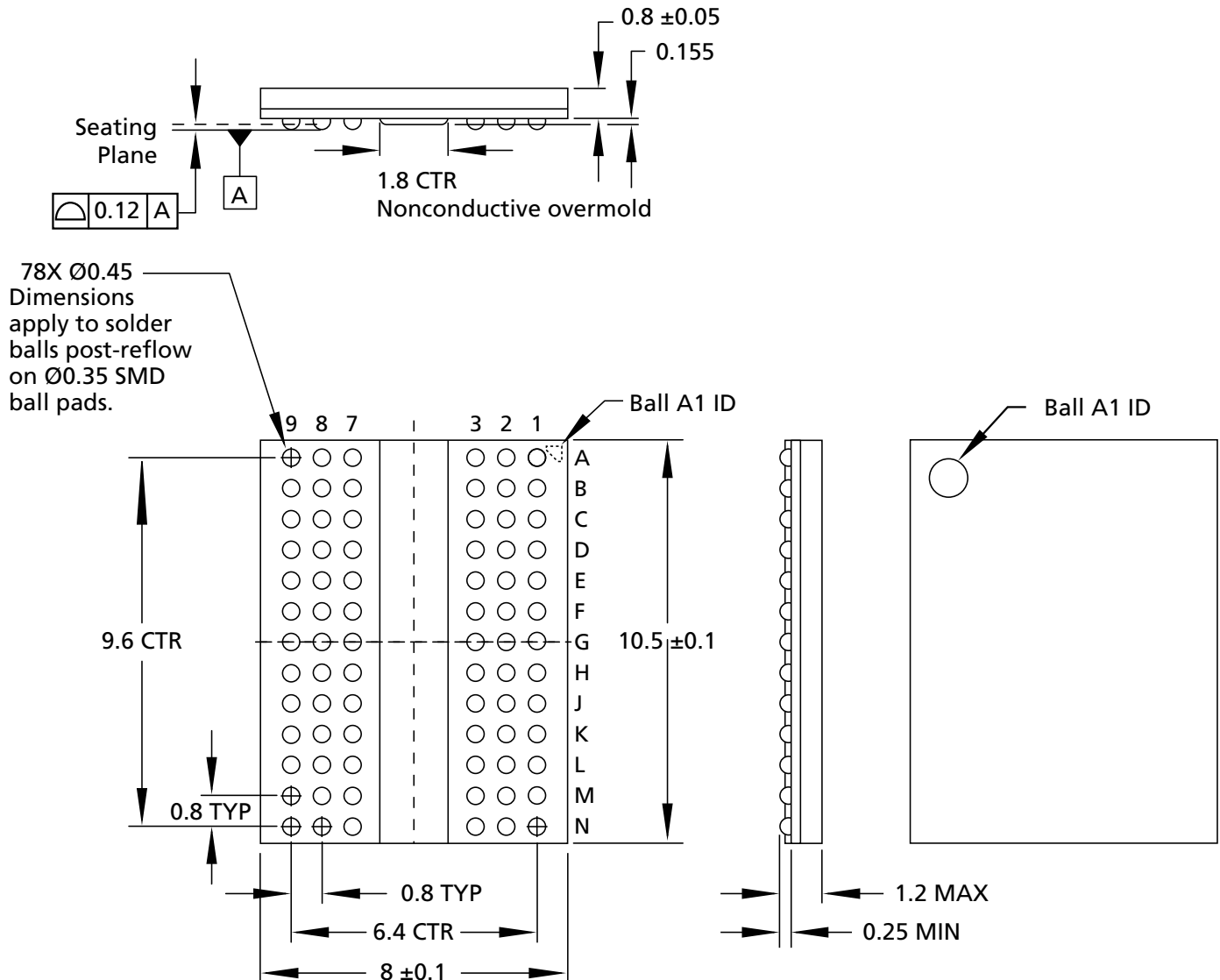
Figure 5: 78-Ball FBGA – x4, x8 (DA)
