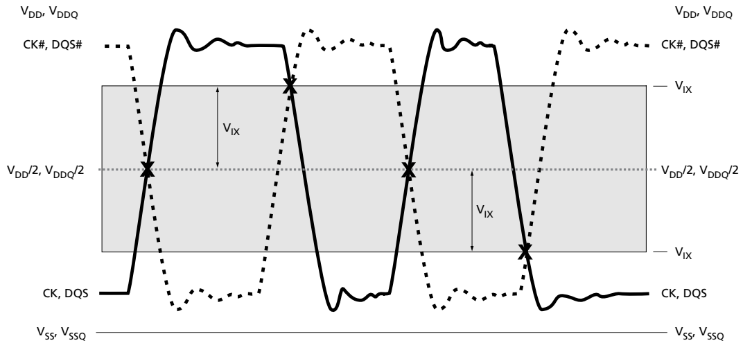
Figure 12: Single-Ended Requirements for Differential Signals
