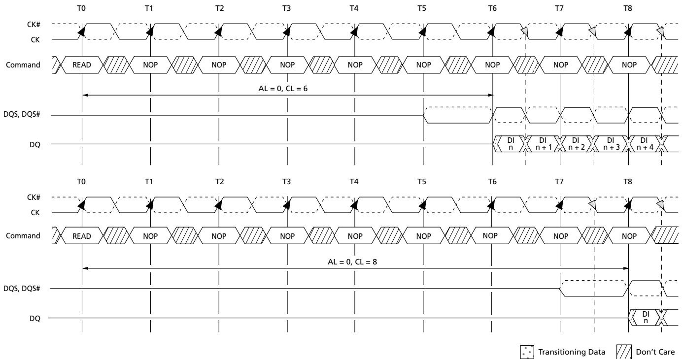
Figure 47: READ Latency
