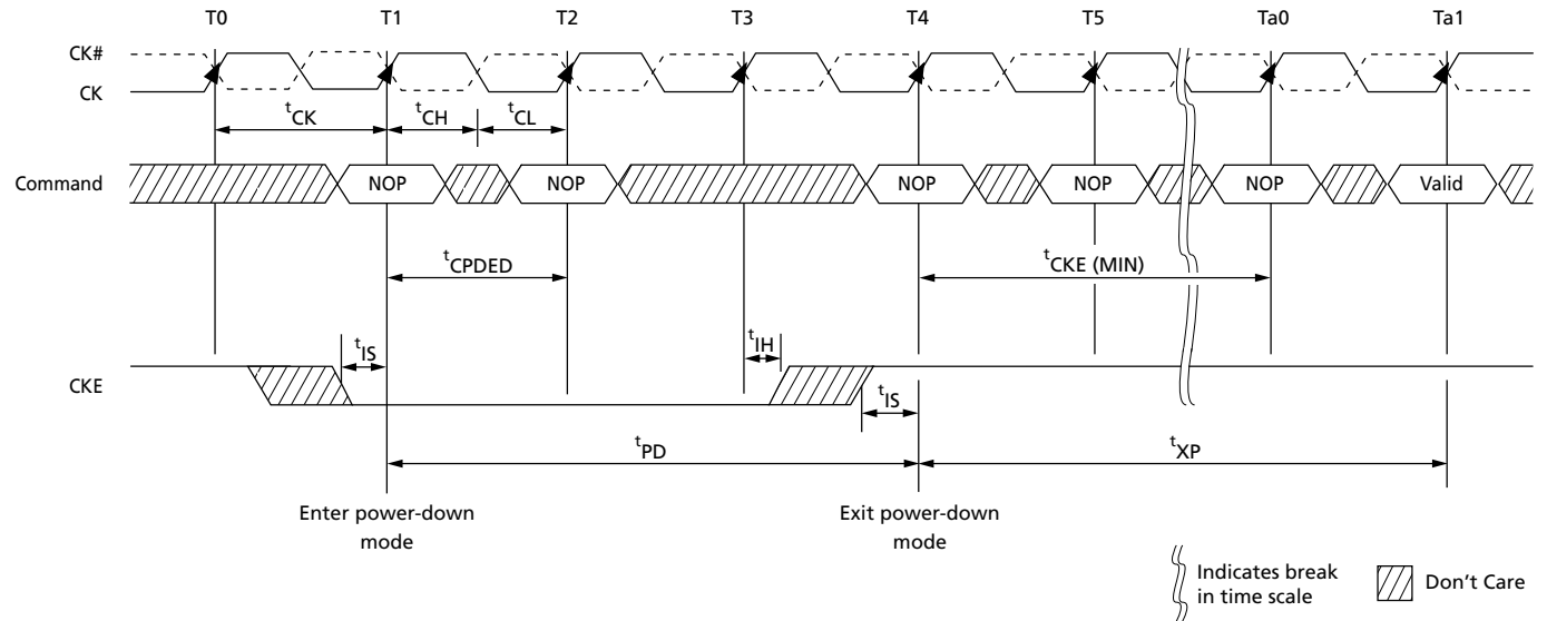
Figure 91: Precharge Power-Down (Fast-Exit Mode) Entry and Exit
