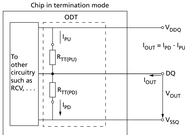
Figure 16: ODT Levels and I-V Characteristics
