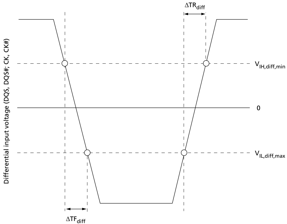
Figure 15: Nominal Differential Input Slew Rate Definition for DQS, DQS# and CK, CK#
