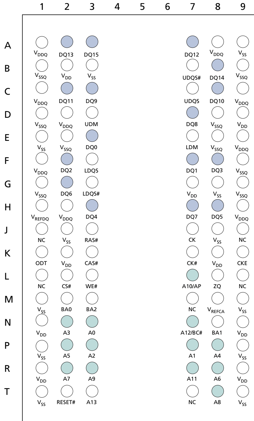
Figure 4: 96-Ball FBGA – x16 (Top View)
