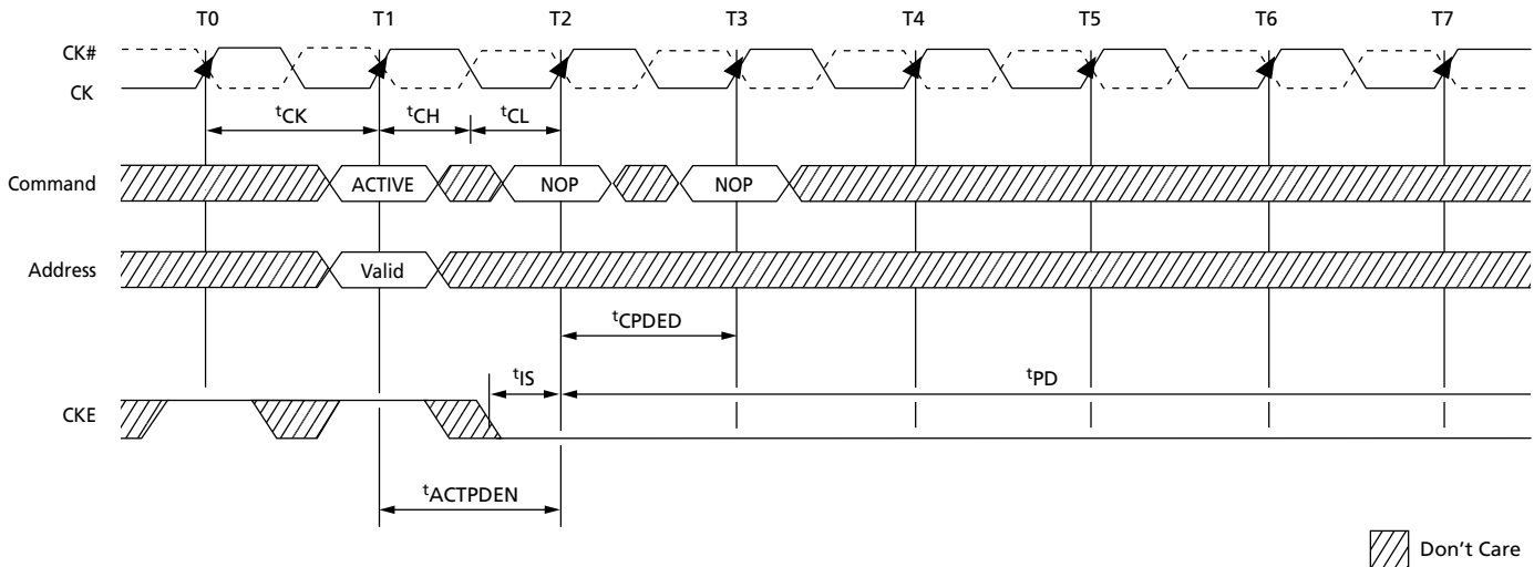
Figure 97: ACTIVATE to Power-Down Entry
