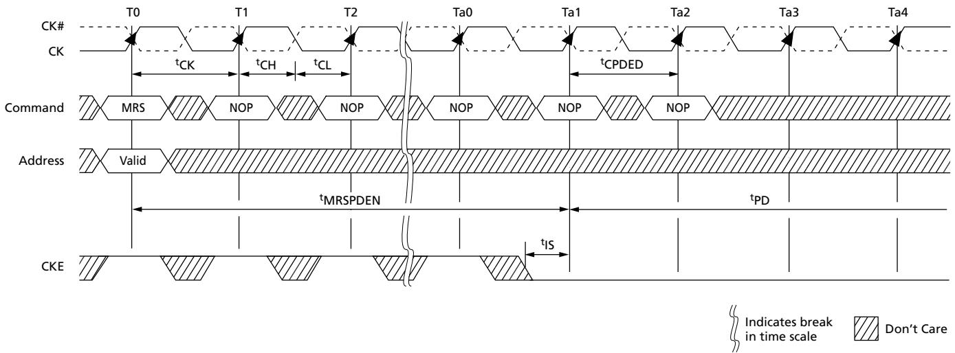
Figure 99: MRS Command to Power-Down Entry
