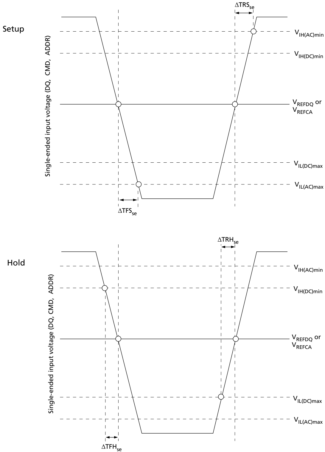
Figure 14: Nominal Slew Rate Definition for Single-Ended Input Signals
