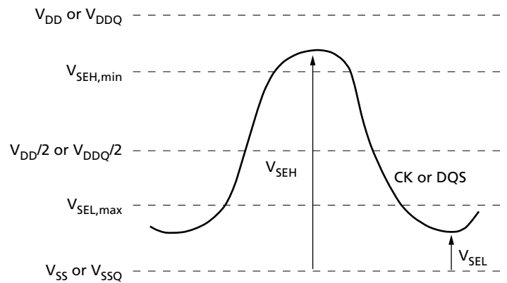
Figure 12: Single-Ended Requirements for Differential Signals
