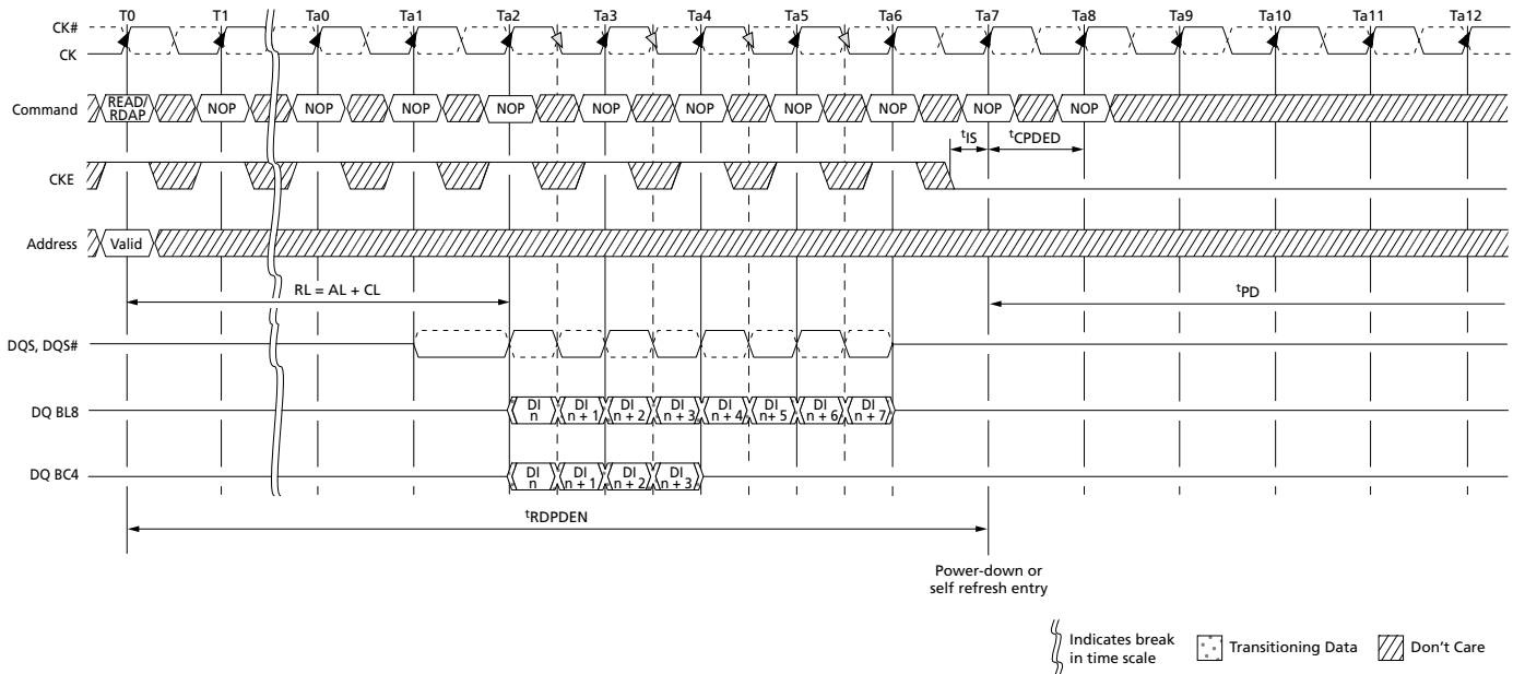
Figure 93: Power-Down Entry After READ or READ with Auto Precharge (RDAP)
