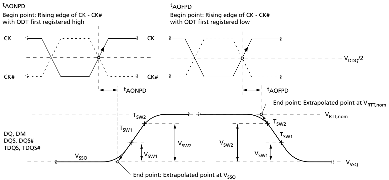
Figure 19: t_{AONPD} and t_{AOFPD} Definitions
