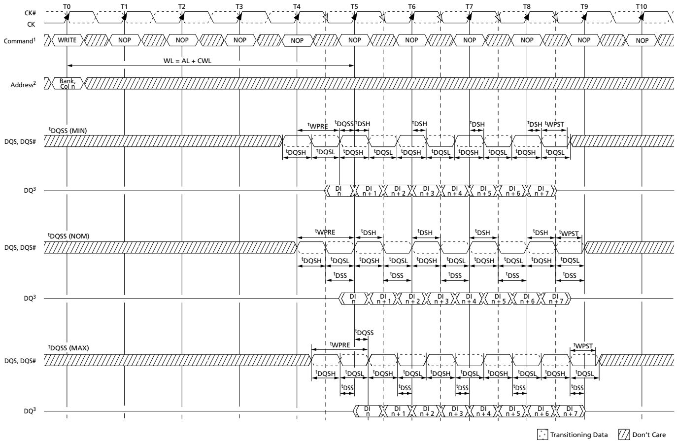
Figure 78: WRITE Burst
