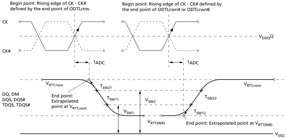
Figure 20: t_{ADC} Definition
