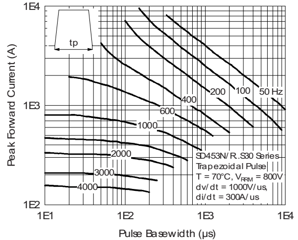
Fig. 33 - Frequency Characteristics
