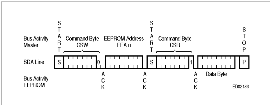
Figure 11 Random Read
