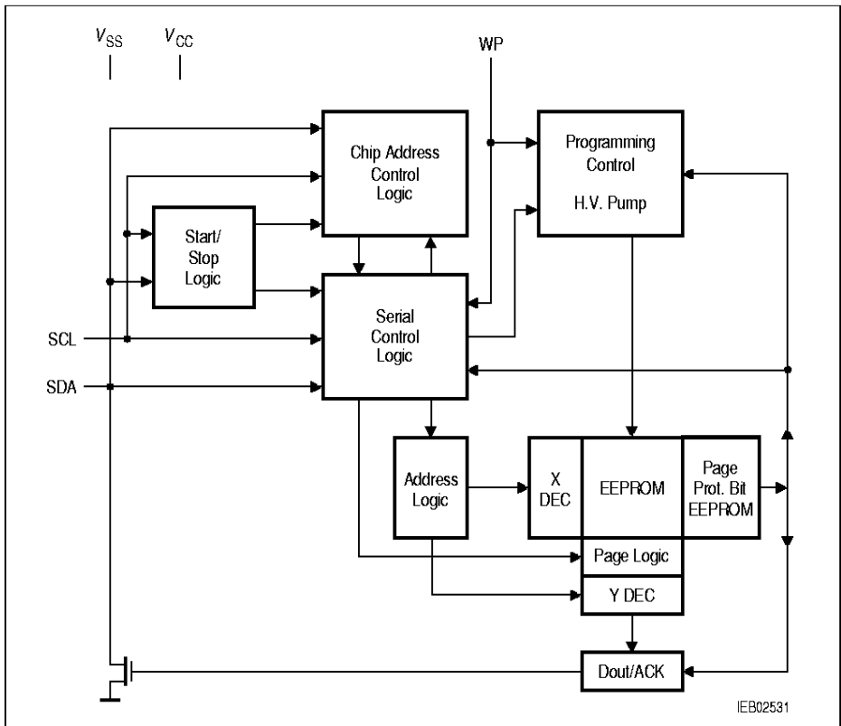
Figure 2 Block Diagram
