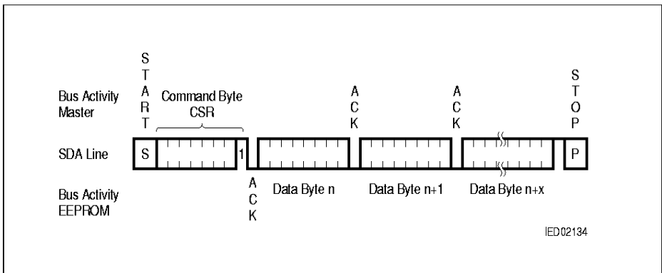
Figure 13 Sequential Read
