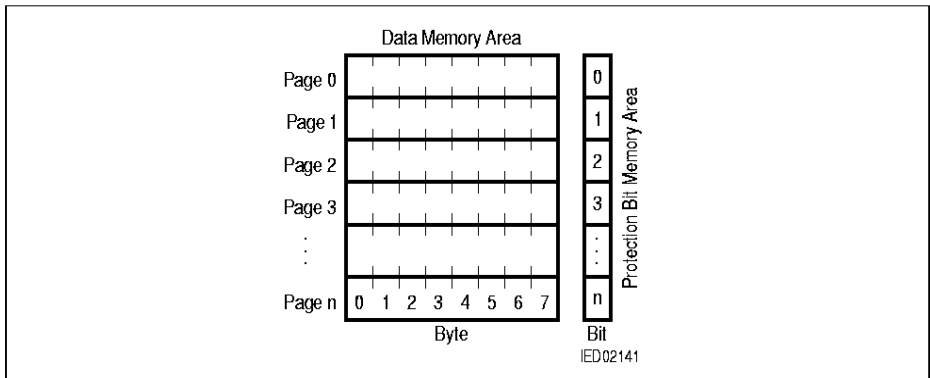
Figure 14 Data Page and Assigned Protection Memory
