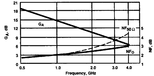
NOISE FIGURE AND ASSOCIATED GAIN vs. FREQUENCY VCE = 8 V, IC = 5 mA
