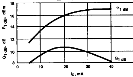
OUTPUT POWER AND 1 dB COMPRESSED GAIN vs. COLLECTOR CURRENT VCE = 8 V, f = 2.0 GHz
