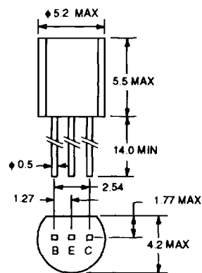
PACKAGE OUTLINE 32
