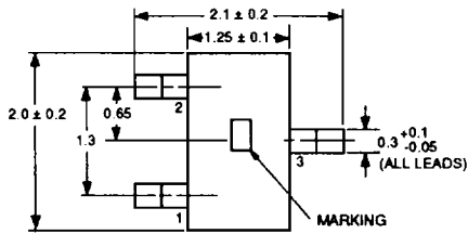
PACKAGE OUTLINE 30
