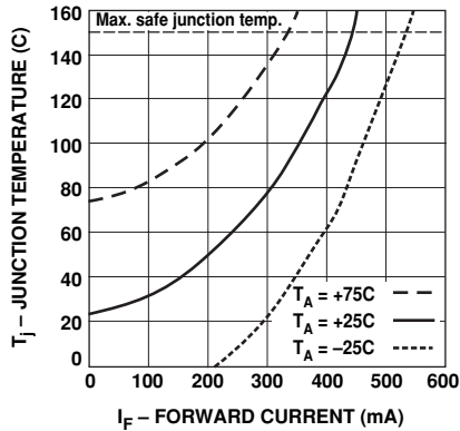
Figure 4. Junction Temperature vs. Current as a Function of Heat Sink Temperature for HBAT-540B and HBAT-540C. Note: Data is calculated from SPICE parameters.
