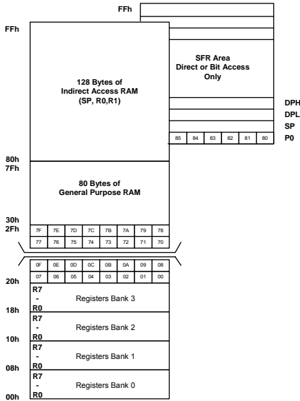
FIGURE 5: VRS51x570 / VRS51x580 INTERNAL LOWER 256 BYTES SRAM STRUCTURE
