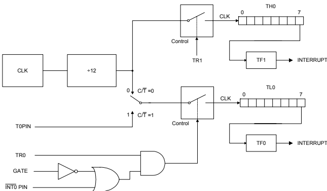
FIGURE 13: TIMER/COUNTER 0 MODE 3
