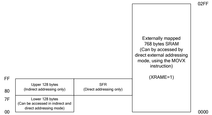
FIGURE 4: VRS51x570 / VRS51x580 SRAM MEMORY
