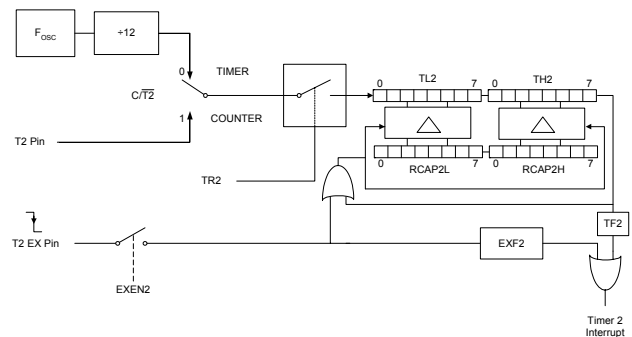
FIGURE 15: TIMER 2 IN AUTO-RELOAD MODE
