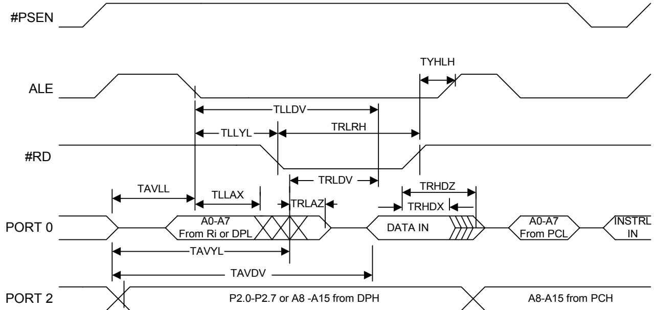
FIGURE 31: EXTERNAL DATA MEMORY READ CYCLE
