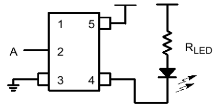
Figure 8. LED Driver
