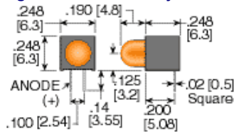
Series PC200 Figure 1. Standard Projection
