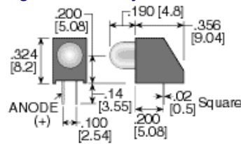
Series PCT220 Figure 2. Low Projection
