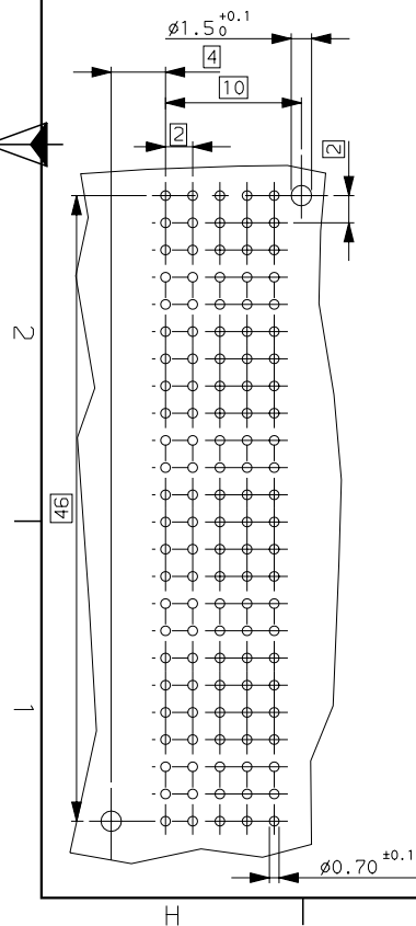
LAYOUT FOR P.C.B CONNECTOR SIDE VIEW
