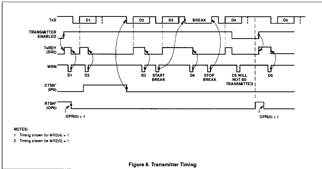
Figure 8. Transmitter Timing
