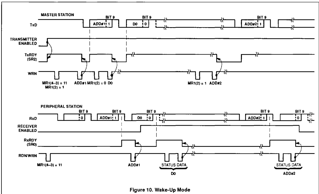
Figure 10. Wake-Up Mode
