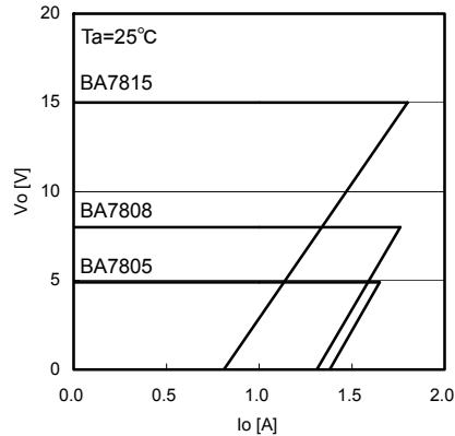
Fig.17 Load Regulation
