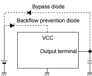
Fig.27 Bypass Diode
