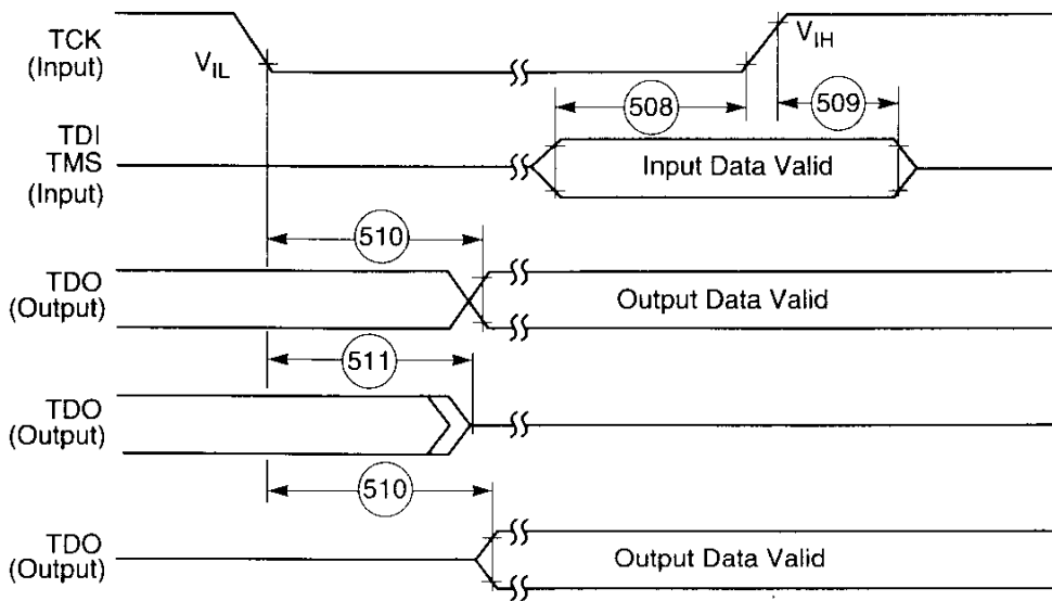
Figure 2-41 Test Access Port Timing Diagram
