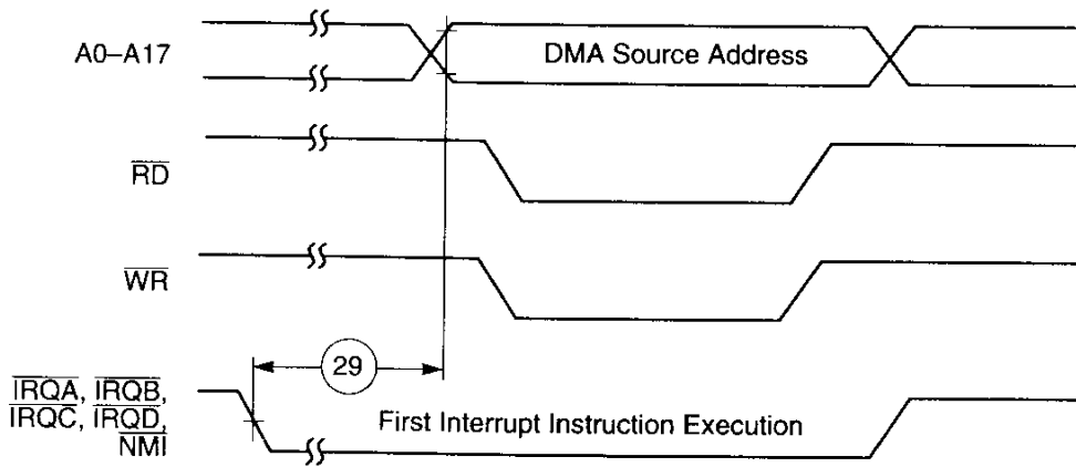
Figure 2-11 External Memory Access (DMA Source) Timing
