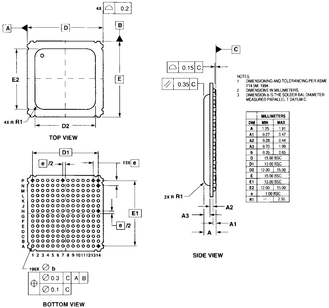
Figure 3-6 DSP56302A Mechanical Information, 196-pin PBGA Package
