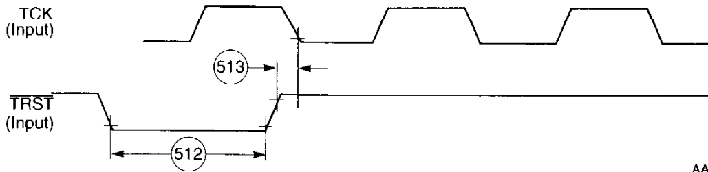
Figure 2-42 \overline{\text{TRST}} Timing Diagram
