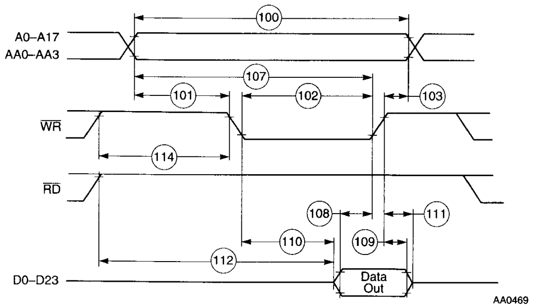
Figure 2-13 SRAM Write Access
