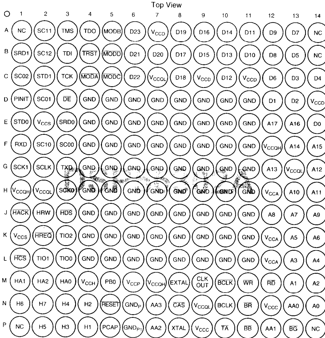
Figure 3-4 DSP56302A Plastic Ball Grid Array (PBGA), Top View
