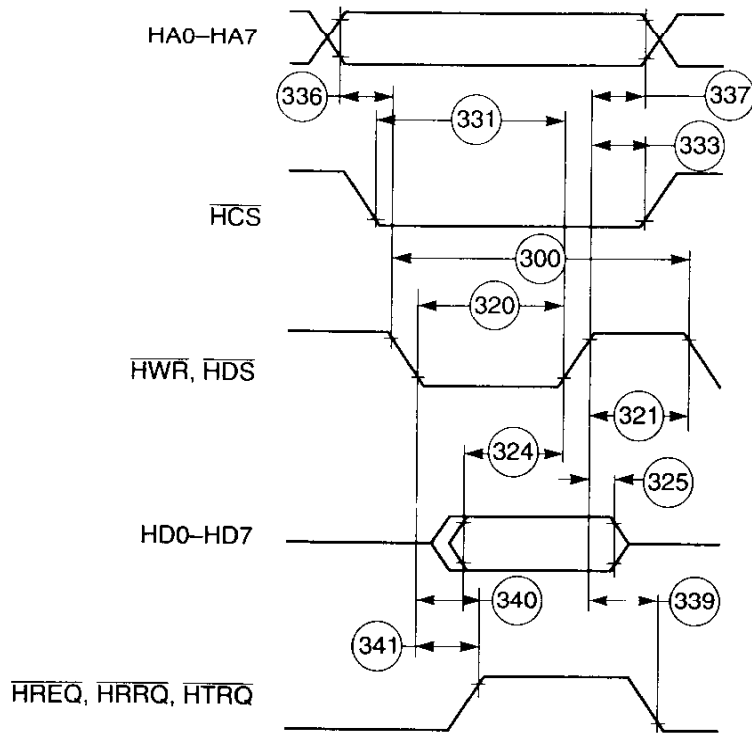
Figure 2-28 Write Timing Diagram, Non-Multiplexed Bus
