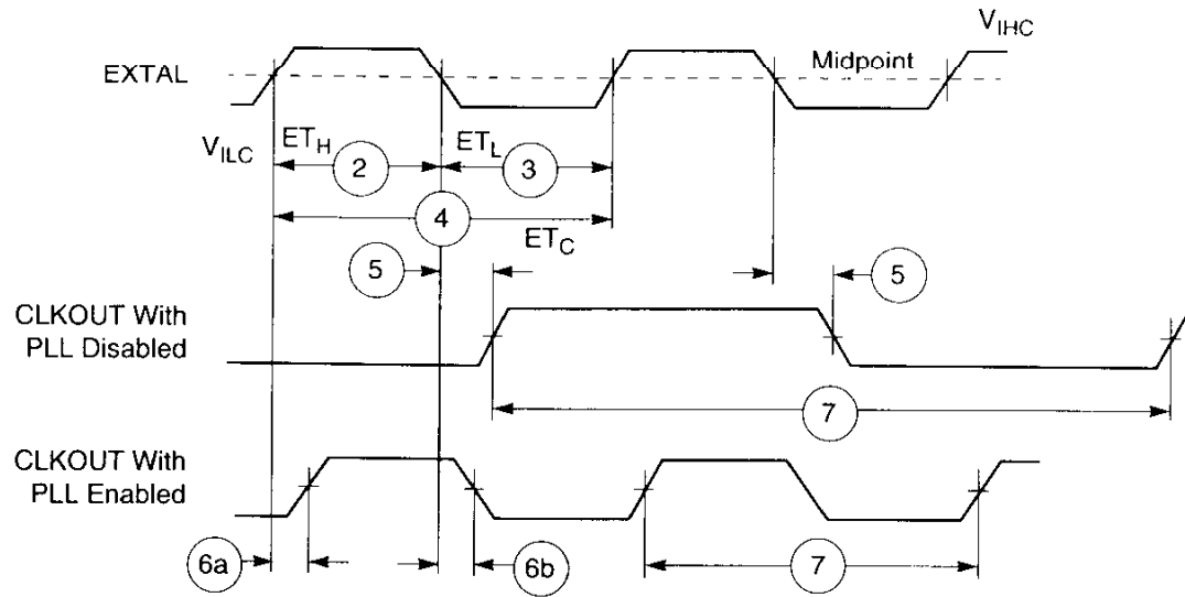
Figure 2-2 External Clock Timing
