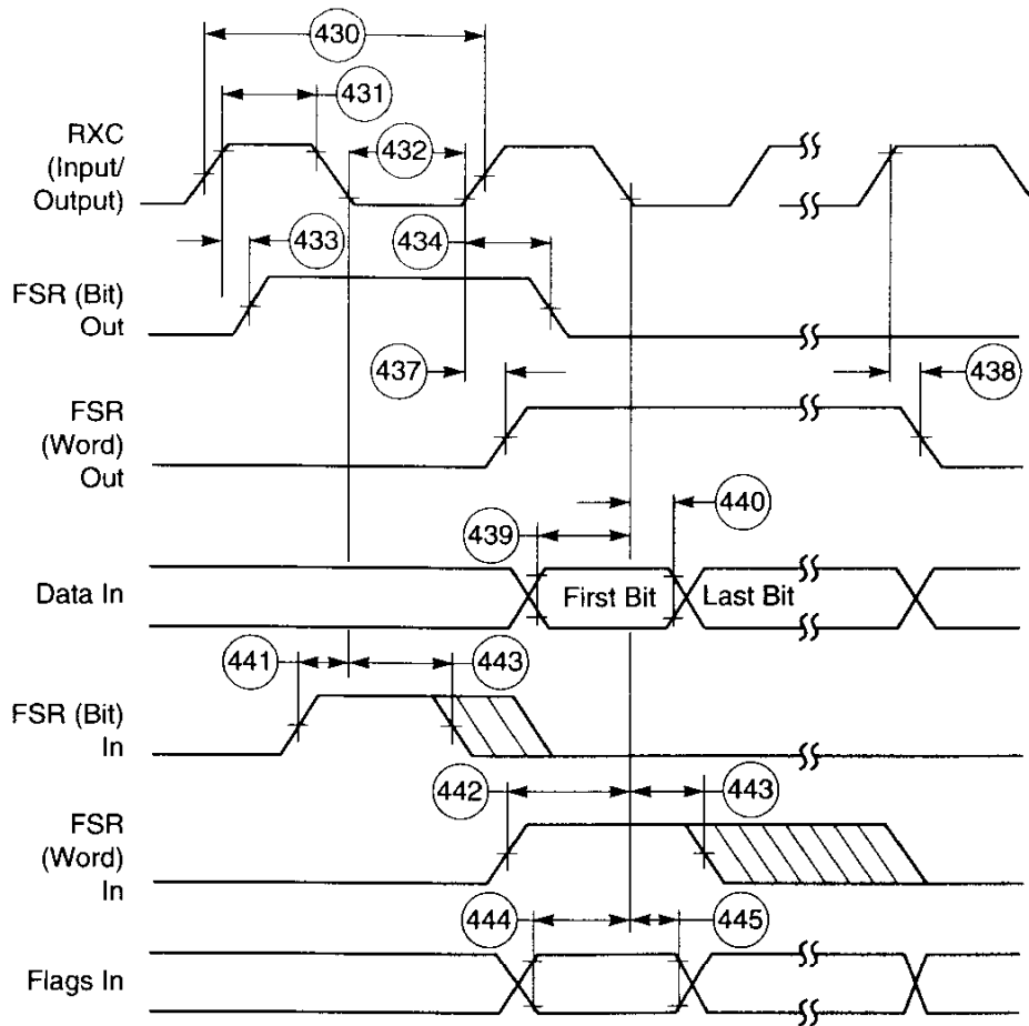
Figure 2-34 ESSI Receiver Timing
