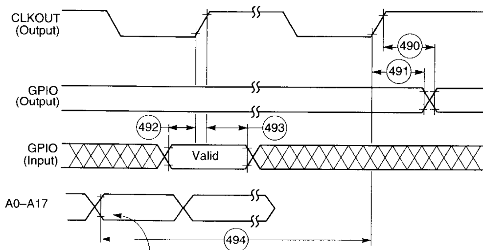
Figure 2-38 GPIO Timing
