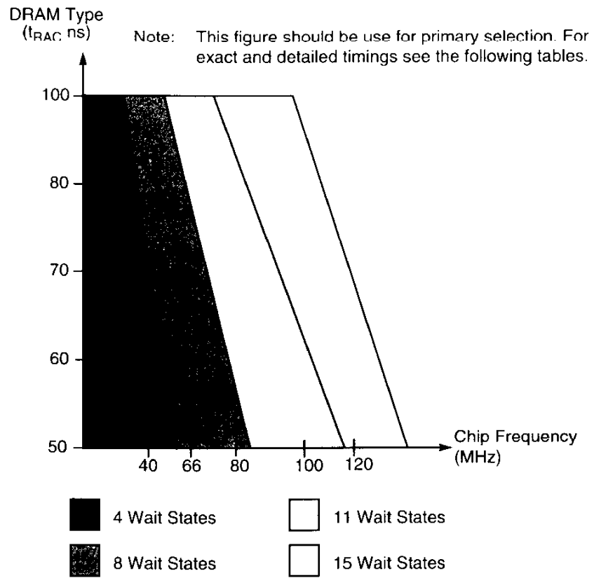
Figure 2-17 DRAM Out-of-Page Wait States Selection Guide
