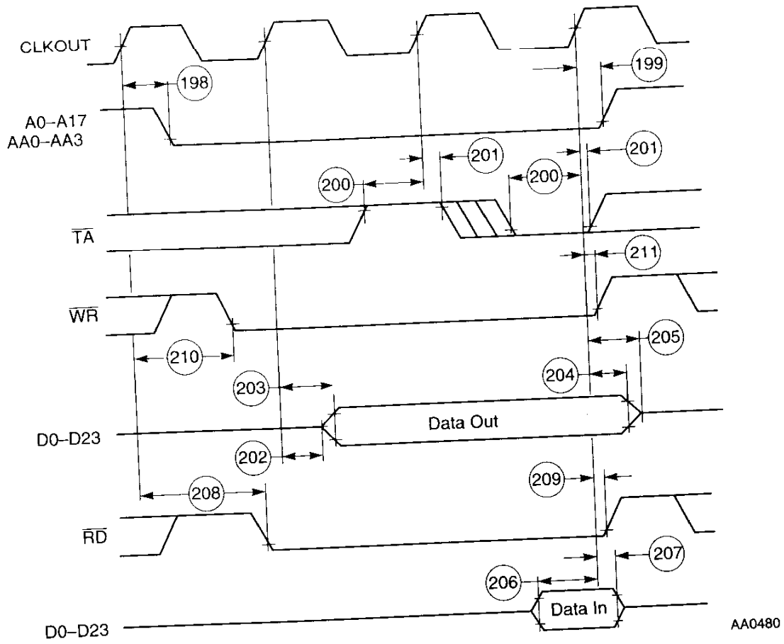
Figure 2-22 Synchronous Bus Timings SRAM 2 WS ( \bar{T}A Controlled)
