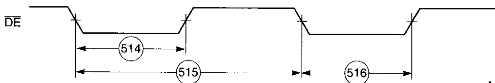
Figure 2-43 OnCE—Debug Request
