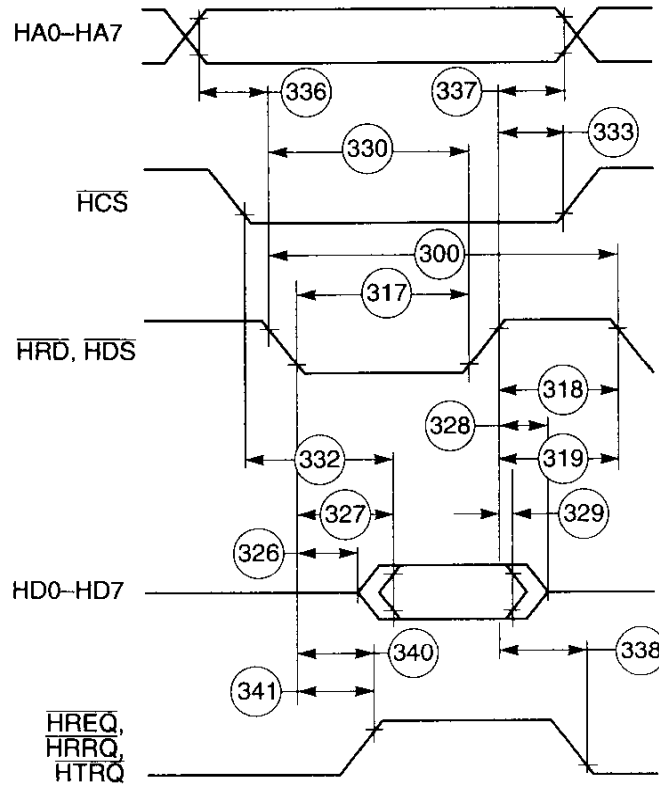
Figure 2-27 Read Timing Diagram, Non-Multiplexed Bus
