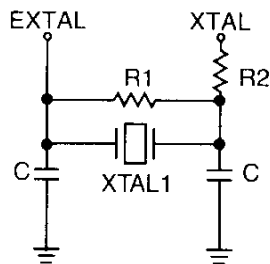
Fundamental Frequency Fork Crystal Oscillator
