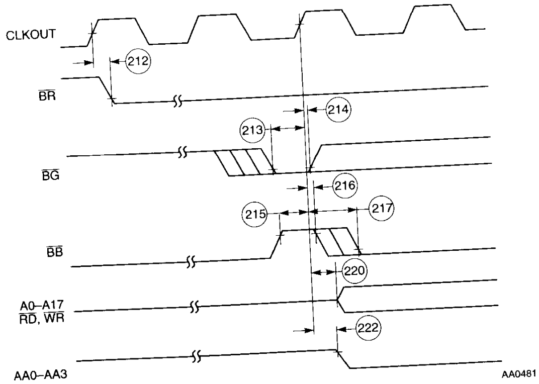
Figure 2-23 Bus Acquisition Timings
