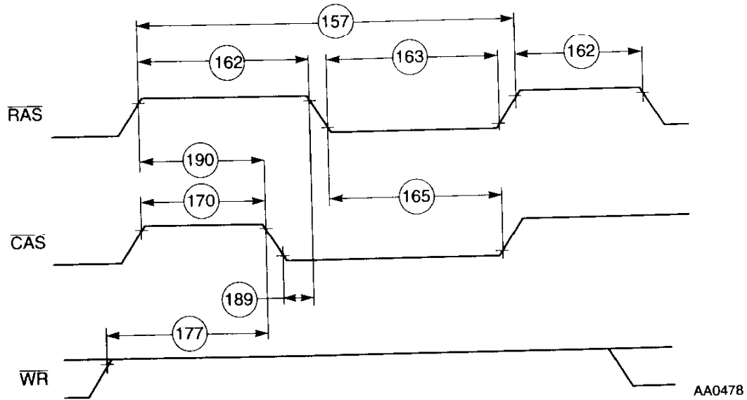
Figure 2-20 DRAM Refresh Access
