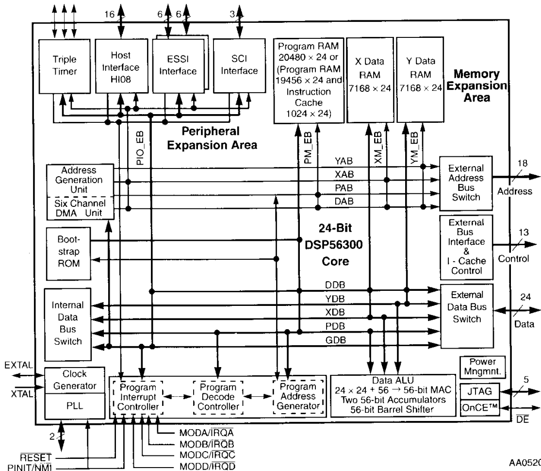
Figure 1 DSP56302A Block Diagram
