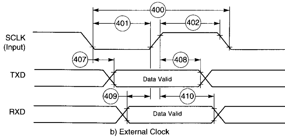
Figure 2-31 SCI Synchronous Mode Timing
