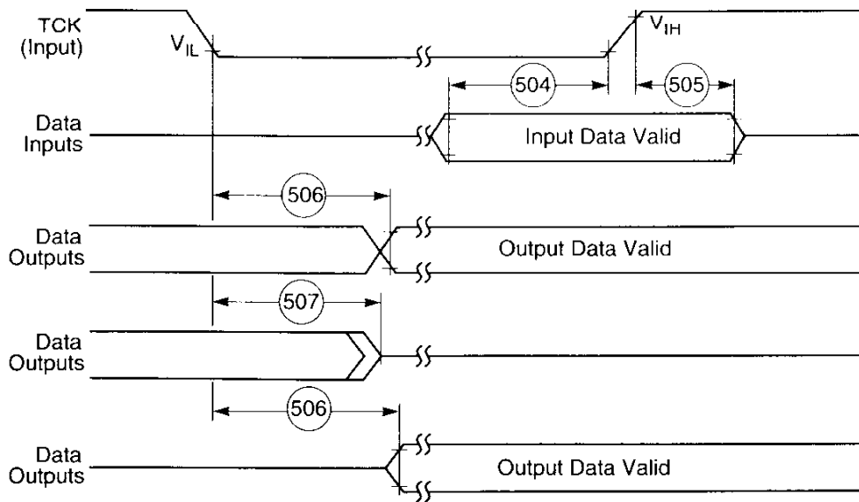
Figure 2-40 Boundary Scan (JTAG) Timing Diagram
