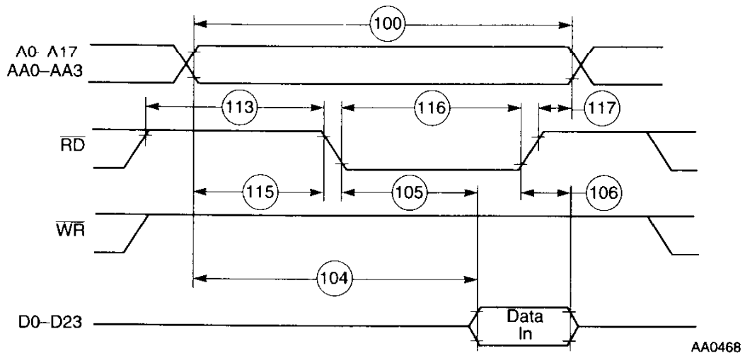
Figure 2-12 SRAM Read Access
