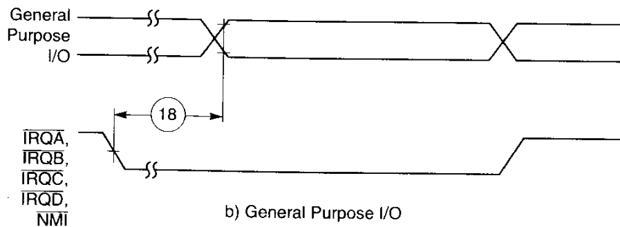
Figure 2-5 External Fast Interrupt Timing
