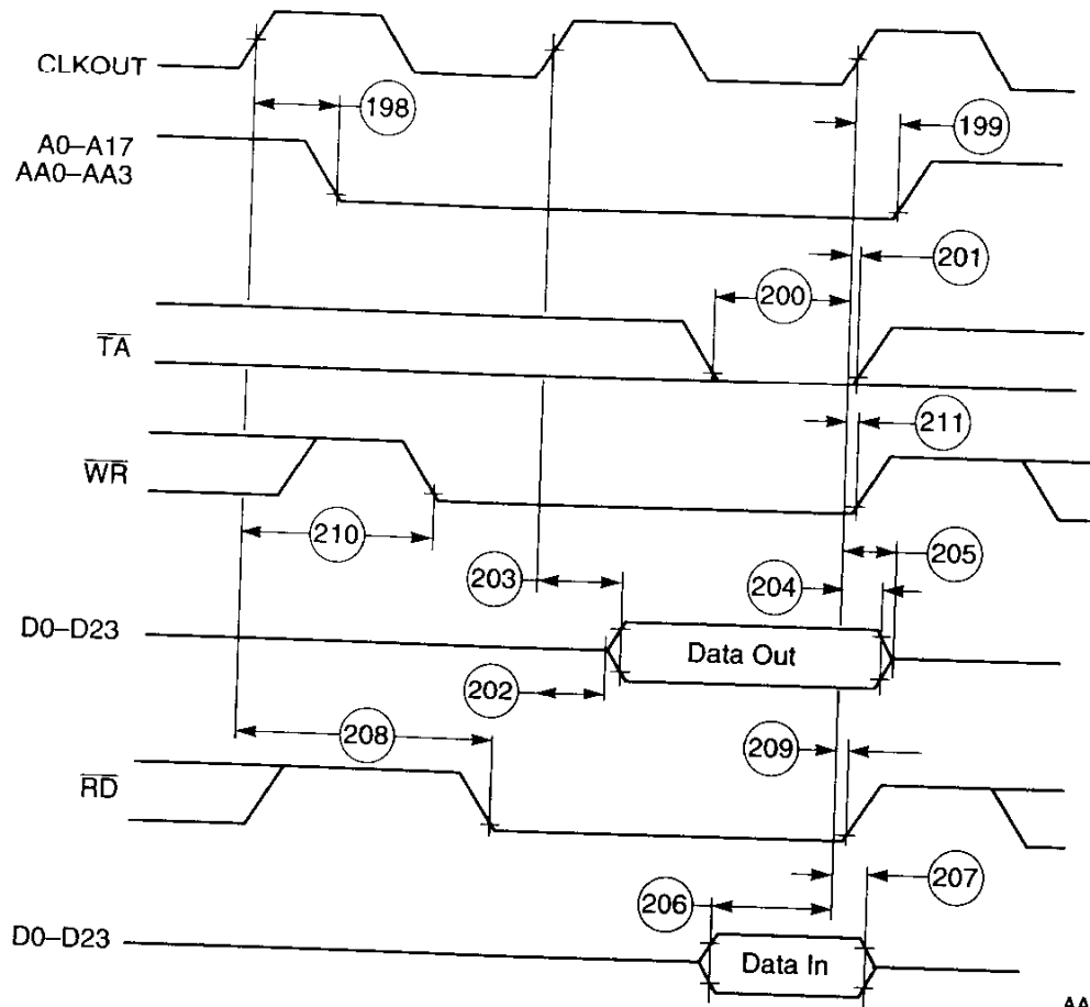
Figure 2-21 Synchronous Bus Timings SRAM 1 WS (BCR Controlled)
