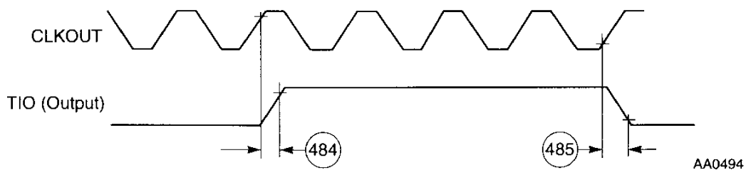
Figure 2-37 External Pulse Generation
