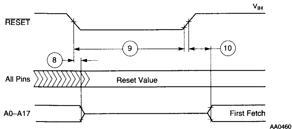
Figure 2-3 Reset Timing
