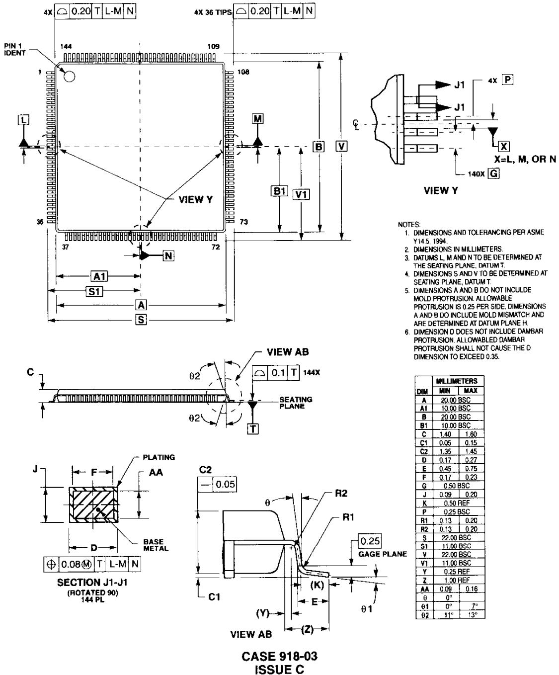
Figure 3-3 DSP56302A Mechanical Information, 144-pin TQFP Package
