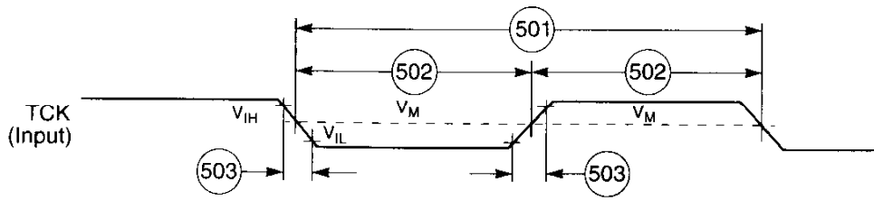
Figure 2-39 Test Clock Input Timing Diagram
