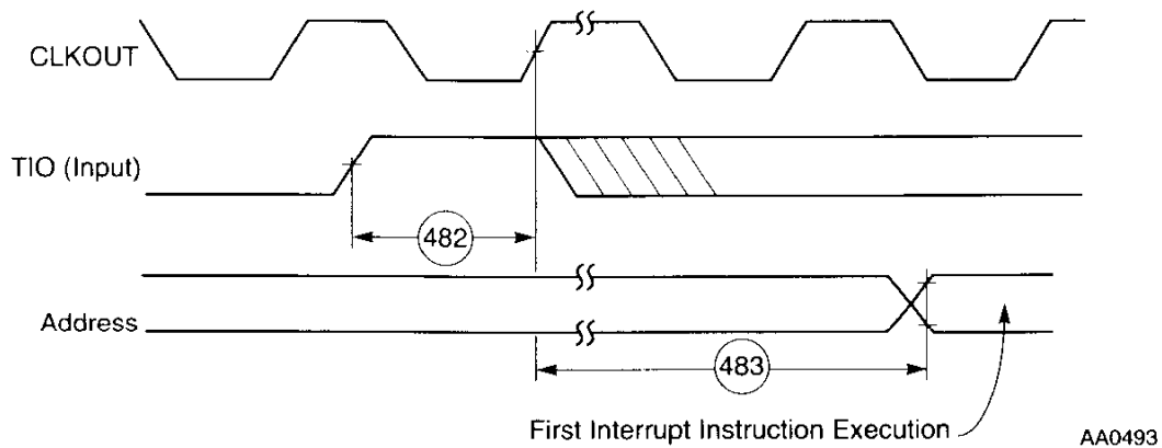
Figure 2-36 Timer Interrupt Generation
