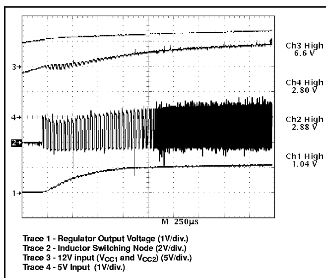
Figure 2: CS-5151H demonstration board startup in response to increasing 12V and 5V input voltages. Extended off time is followed by normal off time operation when output voltage achieves regulation to the error amplifier output.
