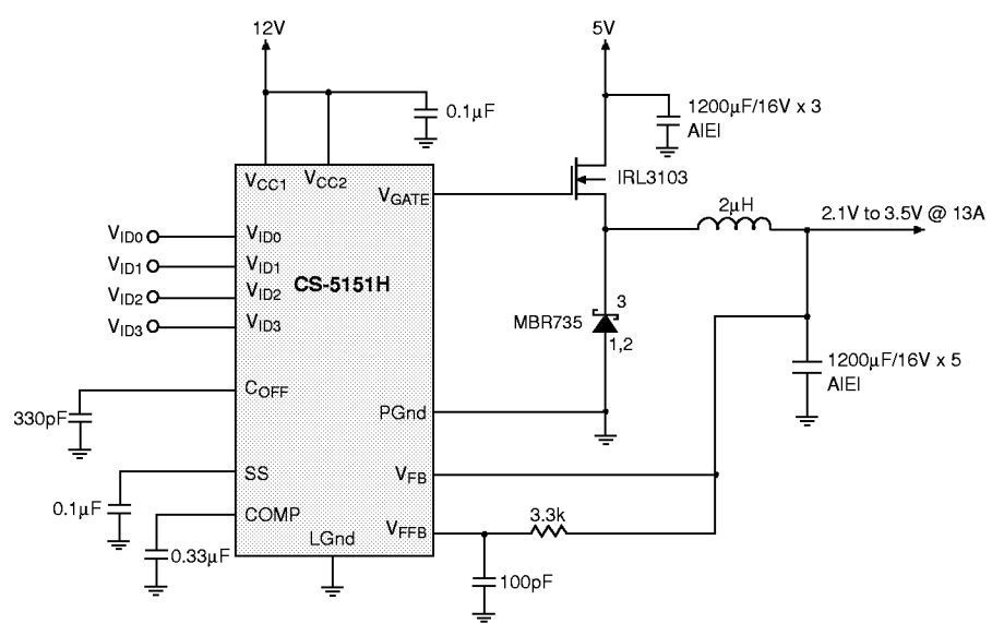
Switching Power Supply for core logic - Pentium® processor with MMX™ Technology
