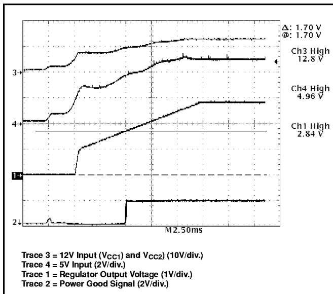
Figure 14: CS-5151H demonstration board during power up. Power Good signal is activated when output voltage reaches 1.70V.
