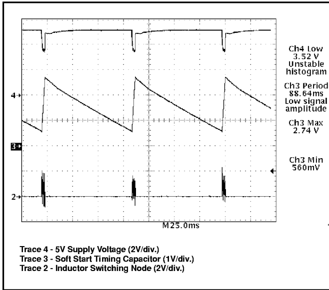
Figure 10: CS-5151H demonstration board hiccup mode short circuit protection. Gate pulses are delivered while the soft start capacitor charges, and cease during discharge.
