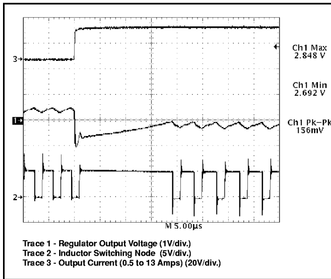
Figure 8: CS-5151H demonstration board response to 13A load turn on (output set for 2.8V). Upon completing a normal off time, the V^2 ™ control loop immediately connects the inductor to the input voltage, providing 100% duty cycle. Regulation is achieved in less than 20µs.
