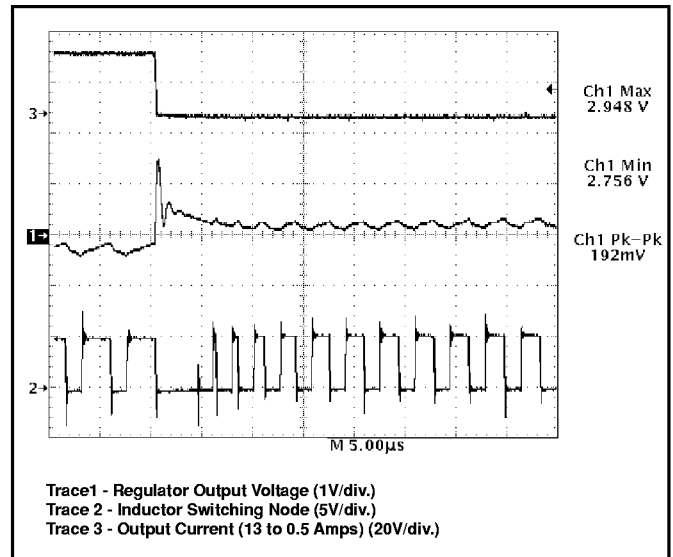
Figure 9: CS-5151H demonstration board response to 13A load turn off (output set for 2.8V). V^2 ™ control topology immediately connects inductor to ground, providing 0% duty cycle. Regulation is achieved in less than 10µs.
