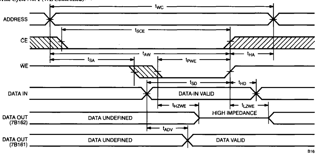
Write Cycle No. 1 ( \overline{WE} Controlled) [10]
