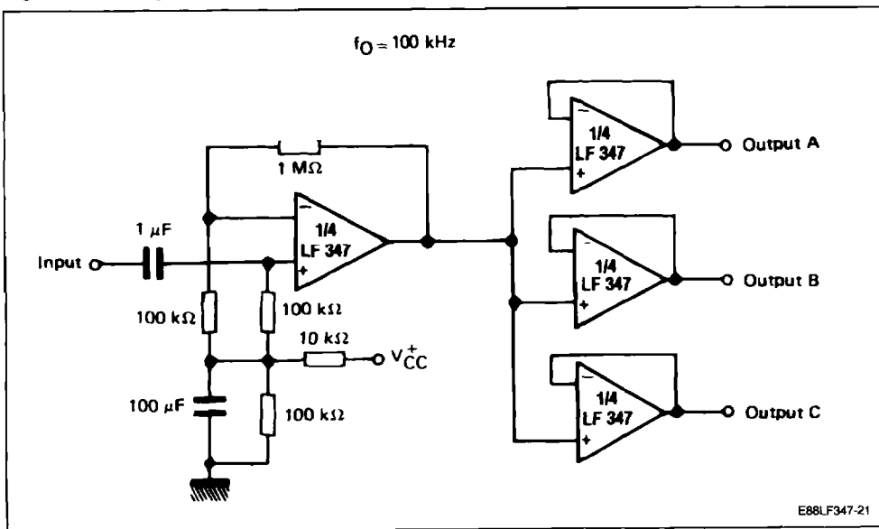
Figure 3 : Voltage Follower.
