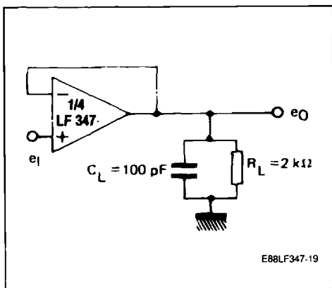
Figure 1 : Voltage Follower.
