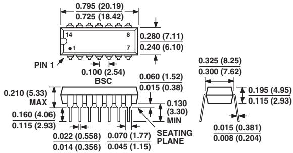
14-Pin Plastic (N) Package (N-14)
