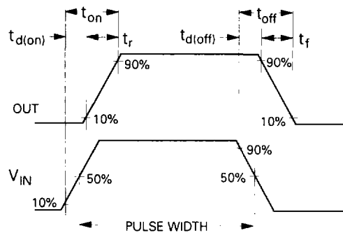
Figure 30. N or P-Channel Switching Waveforms.
