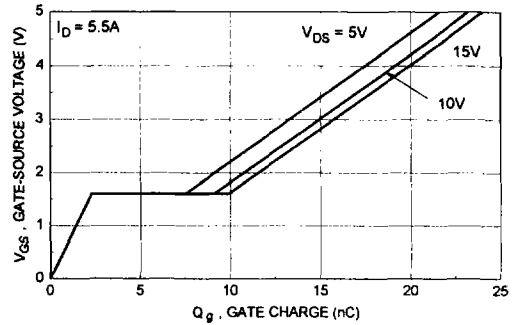
Figure 10. N-Channel Gate Charge Characteristics.
