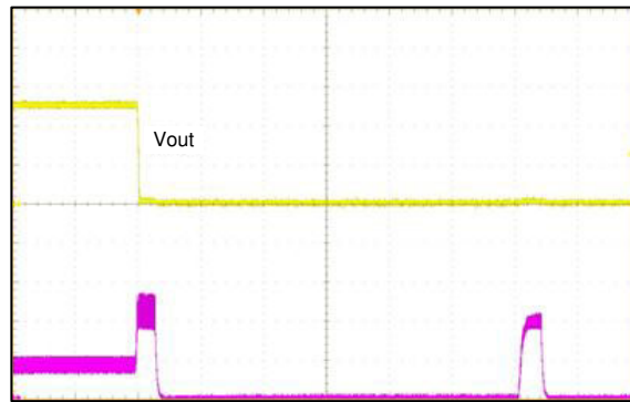
Figure 8-7. Hiccup Operation
