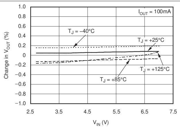
Figure 6-2. Line Regulation
