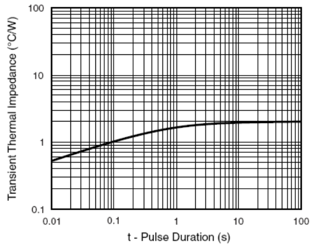
Figure 6. Typical Transient Thermal Impedance Per Diode
